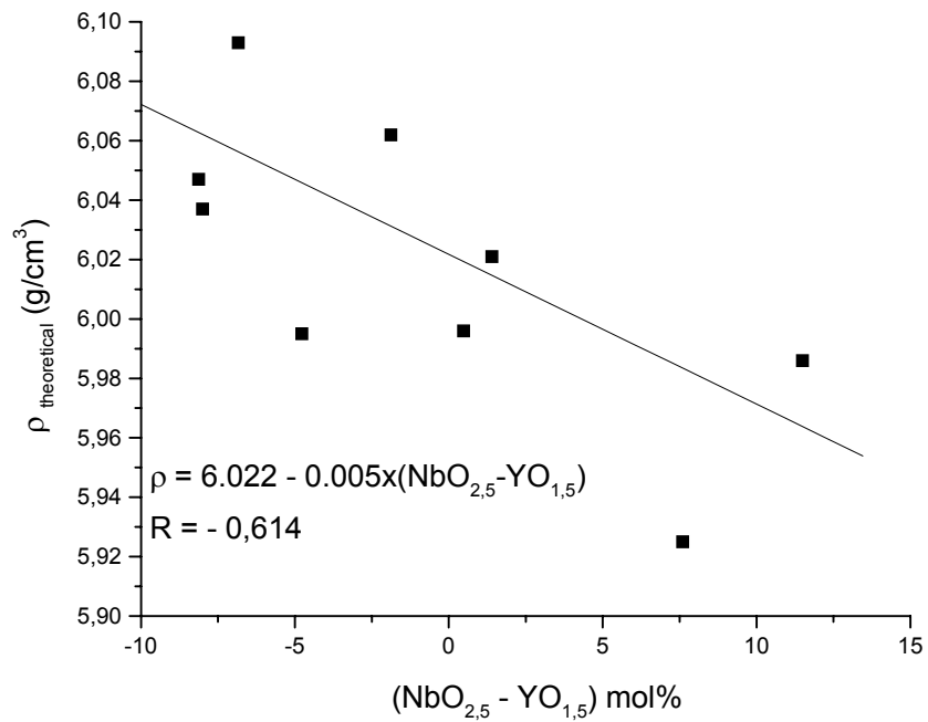
Figure 10: Relation between the difference (\text{NbO}_{2,5} - \text{YO}_{1,5}) mol % and theoretical density.
