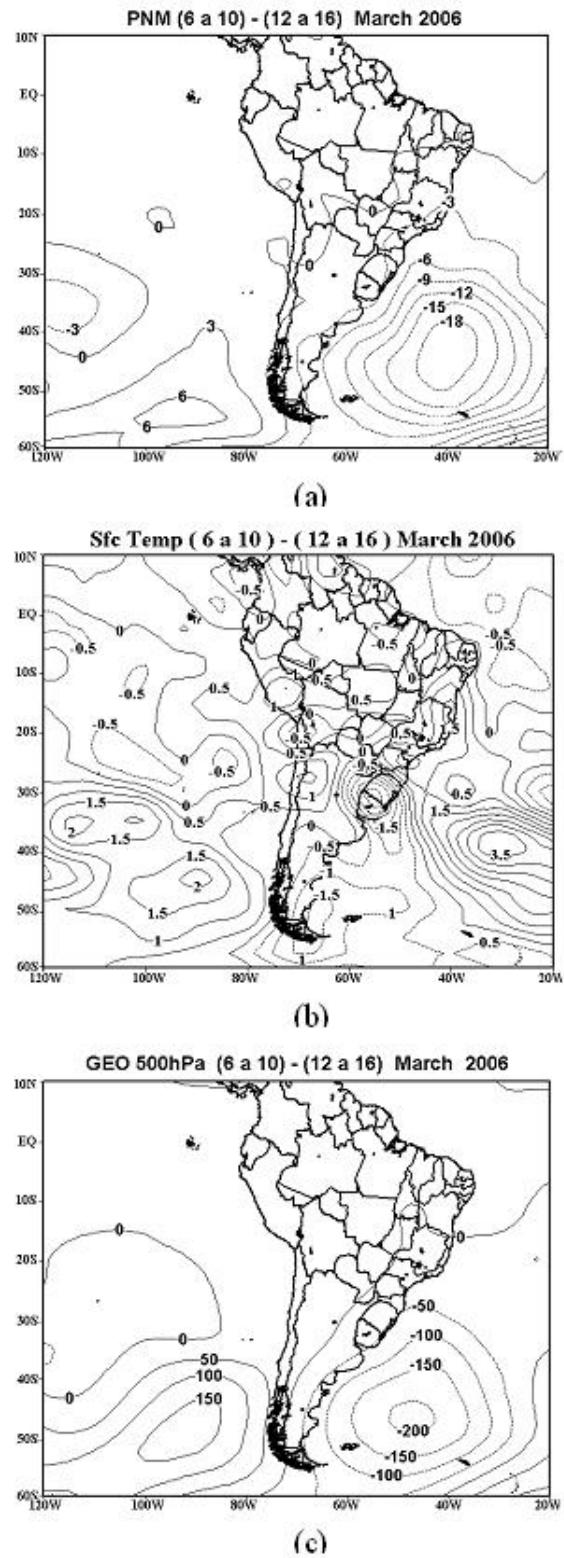
Figure 12 – Differences between rainy and nonrainy episodes. (a) Sea level pressure (hPa), (b) surface temperature (°C), (c) 500 hPa geopotential (m). Broken lines indicate negative values.
