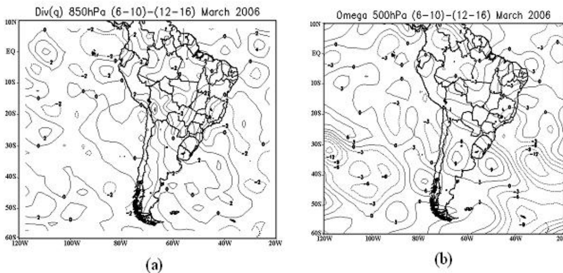
Figure 13 – Differences between rainy and nonrainy episodes. (a) Humidity flux divergence ( 10^{-6} s ^{-1} ), (b) vertical motion (Pa/s). Broken lines indicate negative values.
