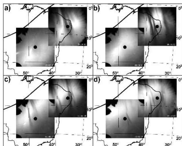
Fig. 7. Evolution of the bubbles structures observed simultaneously from Brasilia and Cariri during the following night (1–2 October) over the same time interval as Fig. 6. Note the lack of structure above Brasilia during the first two hours (panels a and b).
