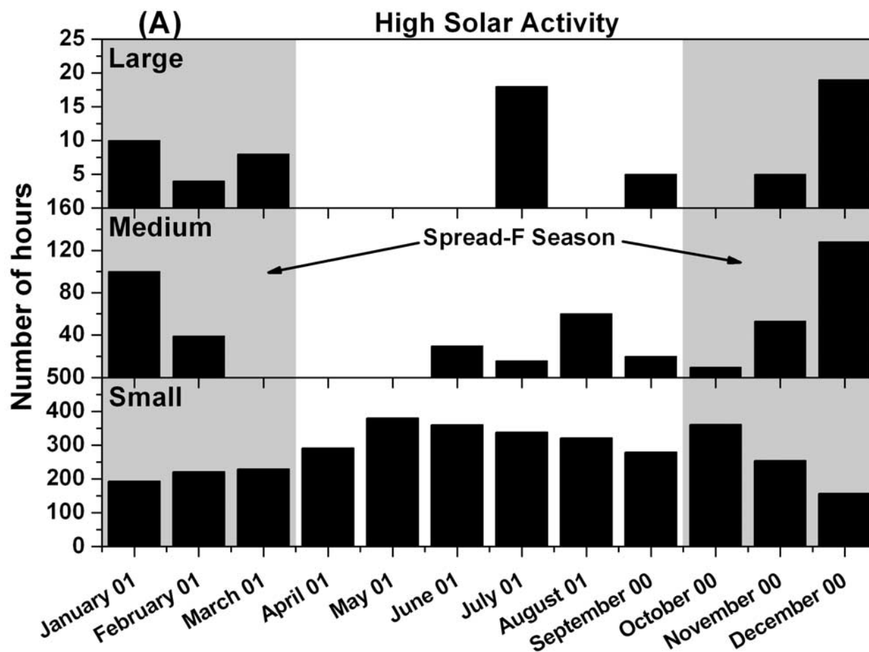
Figure 3. (a) Monthly variations of gravity wave occurrences from September 2000 to August 2001 (high solar activity) for large, medium, and small amplitude oscillations and (b) January 2006 to December 2006 (low solar activity). The gray portions indicate the high season spread F (January to March and October to December).
