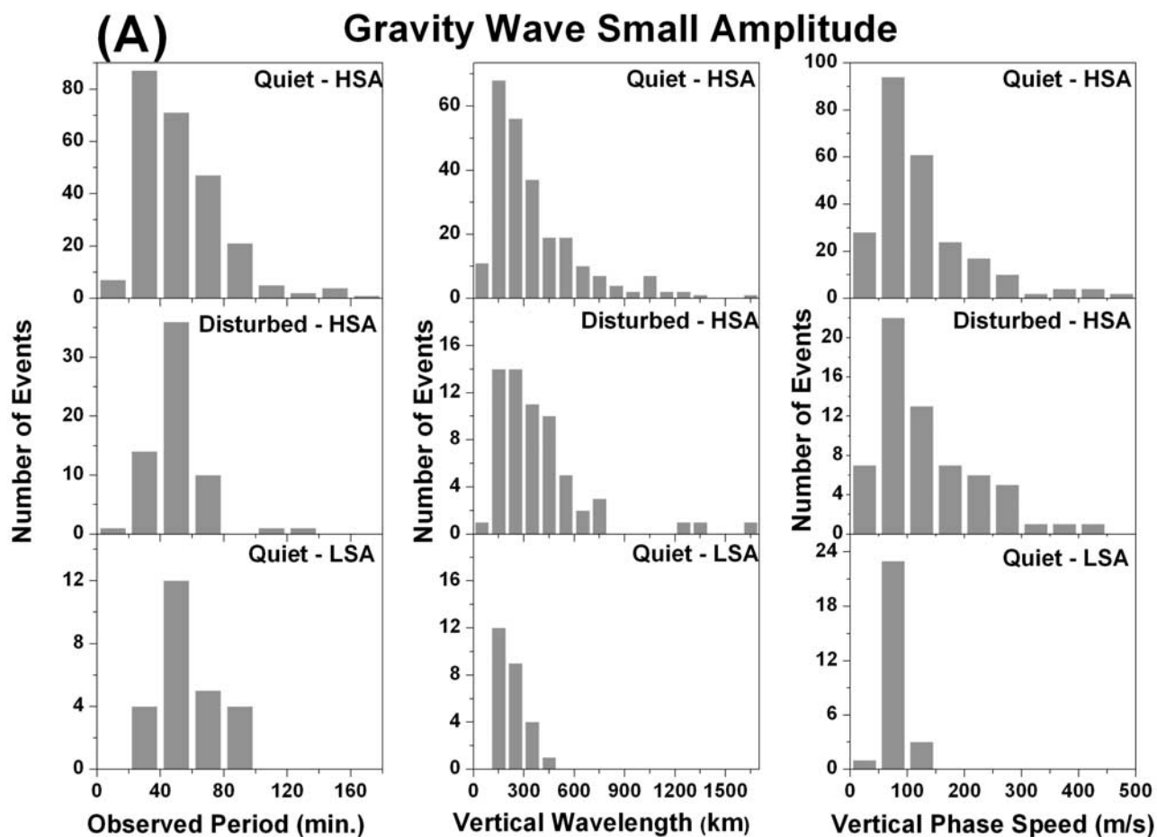
Figure 4. Gravity wave parameters obtained from the oscillations induced in the F_2 layer virtual height. (a) The observed period, vertical wavelength, and phase speed for the small-amplitude gravity waves, measured on quiet and disturbed days during high solar activity and quiet days during low solar activity. (b) The parameters for medium/large amplitude gravity waves observed in the same period shown in Figure 4a.
