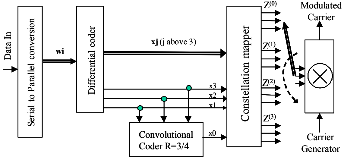
Figure 3-31: Structure of the 4D 8PSK-TCM Coder/Mapper
