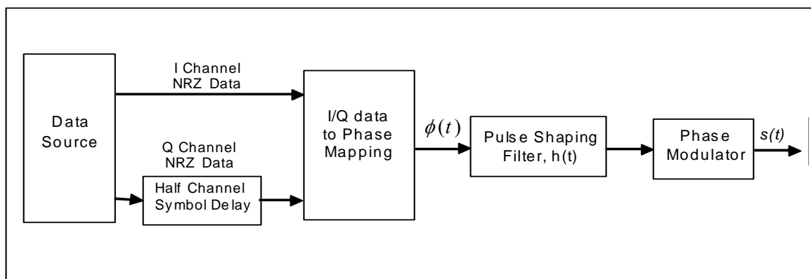
Figure 3-19: Filtered OQPSK with Linear Phase Modulator (OQPSK/PM)
