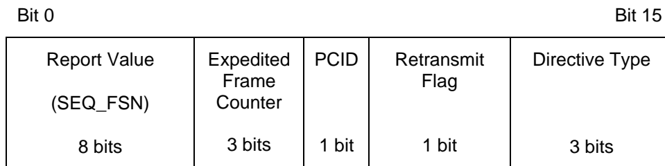
Figure A-7: Proximity Link Control Word
