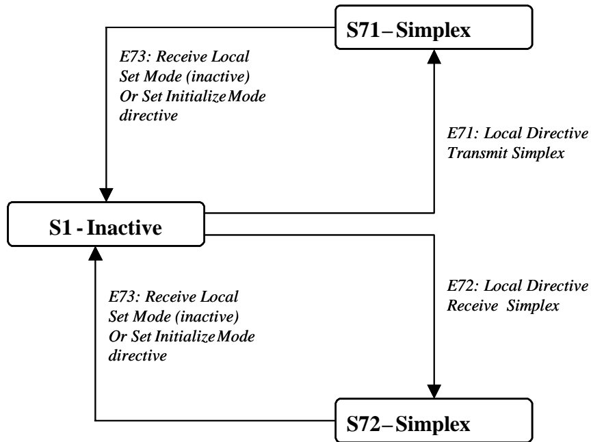
Figure 6-3: Simplex Operations
