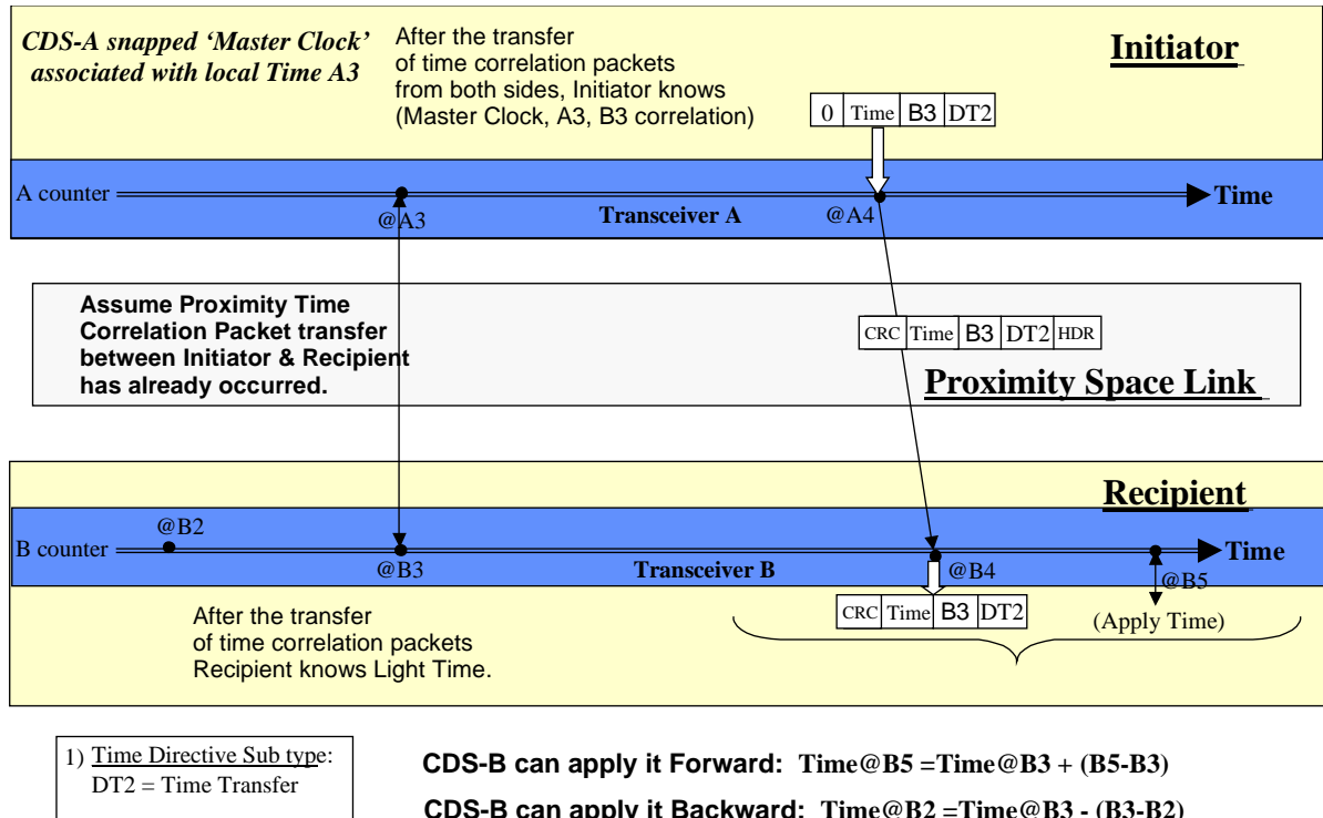
Figure 5-2: Transferring Time to a Remote Asset
