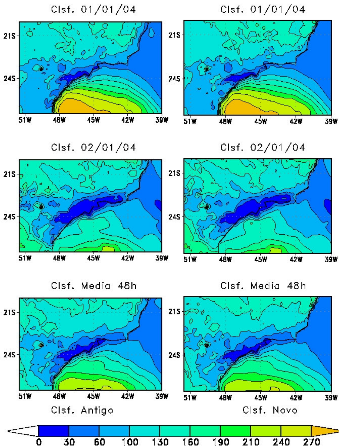
Figura 9: CALOR LATENTE (W/m 2 )
