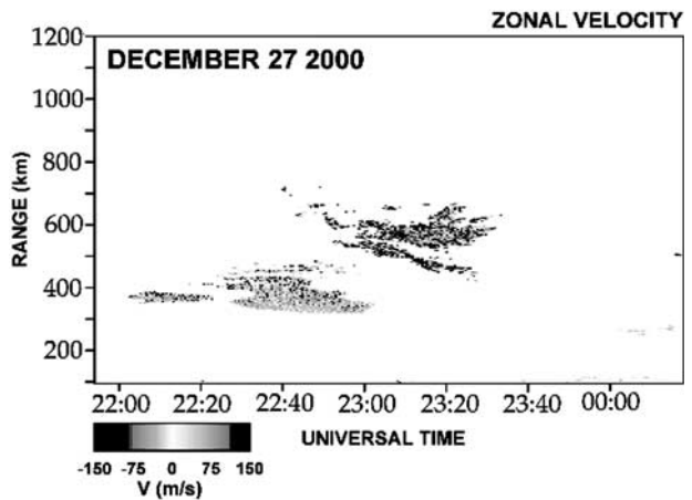
Figure 9. RTI of F region echoes and their vertical (positive upward) and zonal drifts (positive eastward) for December 27, 2000. See color version of this figure at back of this issue.
