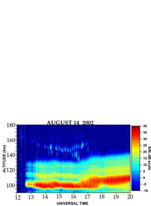
Figure 7. RTI 150 km and electrojet echoes for August 14, 2002.
