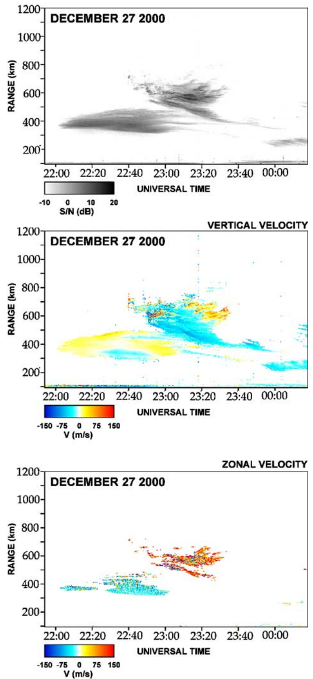
Figure 9. RTI of F region echoes and their vertical (positive upward) and zonal drifts (positive eastward) for December 27, 2000.
