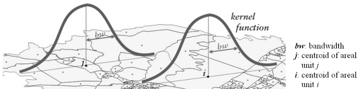
Figure 2. Gaussian kernel estimator.
