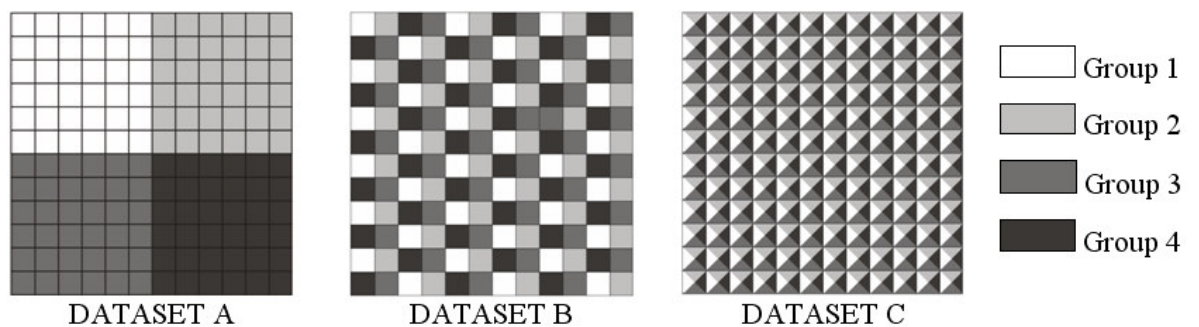
Figure 4. Artificial datasets.
