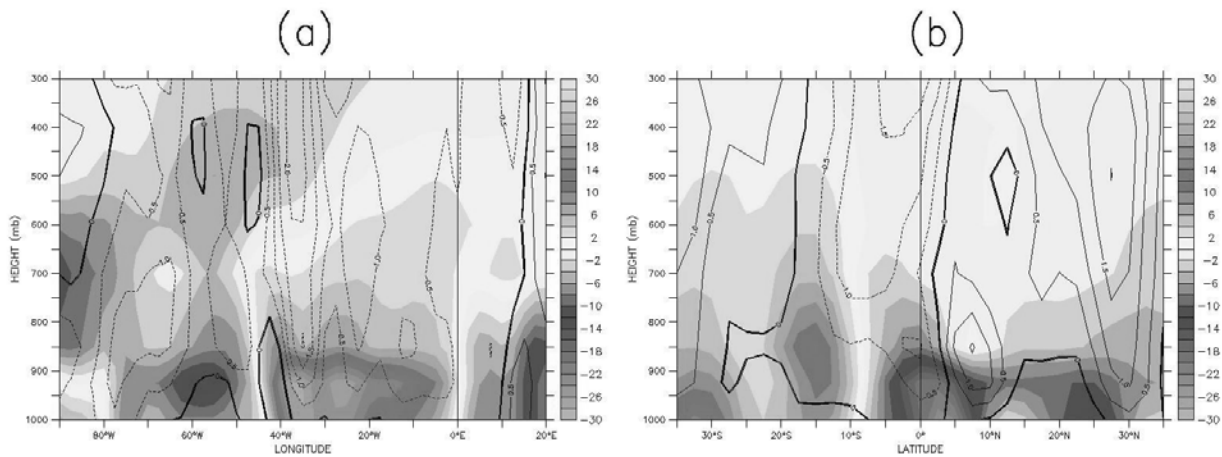
Figure 4: Bias between flood years and drought years (a) of the FMAM zonal moisture flux ( 10^{-3} g/kg.m/s) averaged between 10°S and the equator, and (b) of the FMAM meridional moisture flux ( 10^{-3} g/kg.m/s) averaged between 45°W and 35°W. In both cases the black contours represent the vertical velocity omega ( 10^{-2} Pa/s). Contour interval is 0.5, and negative contours (upward bias) are dashed.
