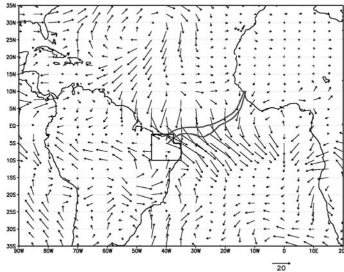
Figure 3: Bias of the FMAM 1000 hPa horizontal moisture flux ( *1000 \text{ g/kg.m/s} ) between flood years and drought years. The blue (red) line indicates the average ITCZ position for FMAM of the five flood (drought) years. The black polygon delimits the region defining NEB.
