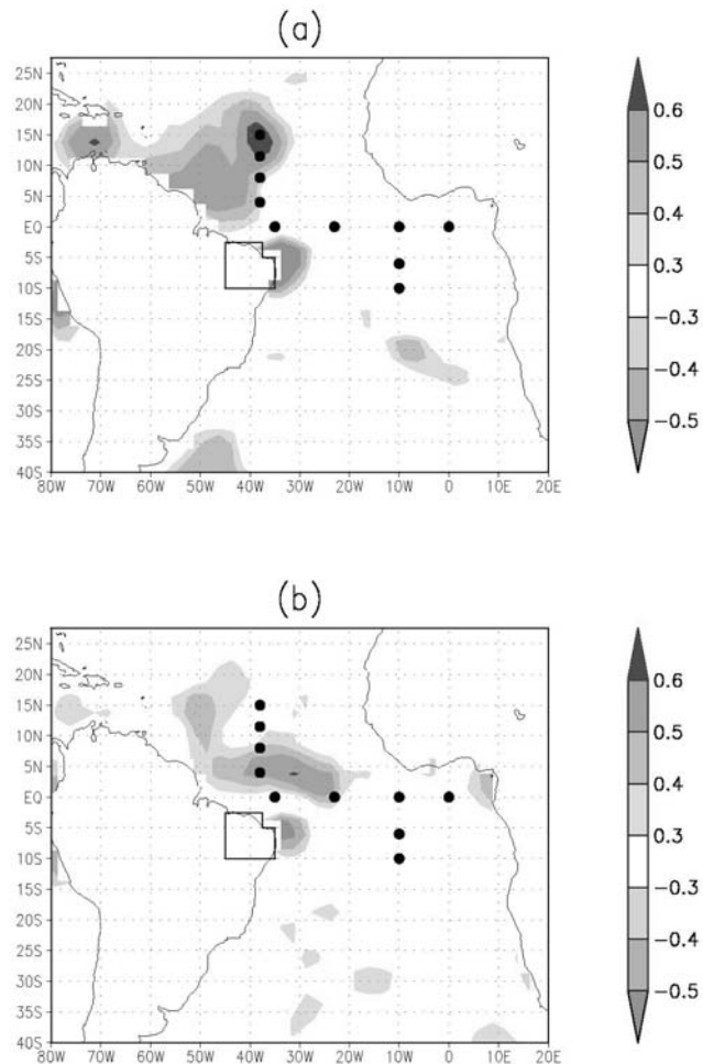
Figure 2: (a) Correlation of the monthly mean anomalous values of NEB convective cloud coverage with the Tropical Atlantic latent heat flux for FMAM during the 1984-1993 period; (b) The same as (a) with the NEB convective cloud cover in the months FMAM and the Tropical Atlantic heat flux in the months JFMA (one month lag). The black polygon delimits NEB, and the full black circles indicate the position of the PIRATA buoys.
