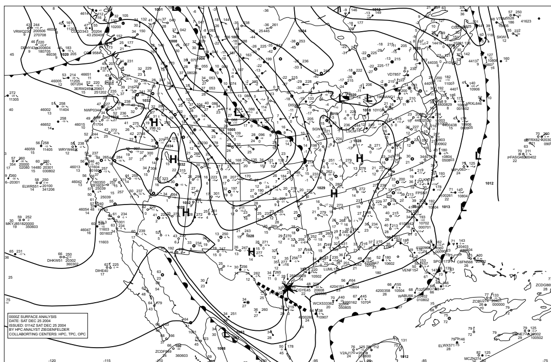
Fig. 8. United States Hydrometeorological Prediction Center surface analysis valid at 0000 UTC 25 December 2004. Star symbol marks the location of the soundings in Figure 10, and the bold, dashed line represents the cross section shown in Figure 11.
