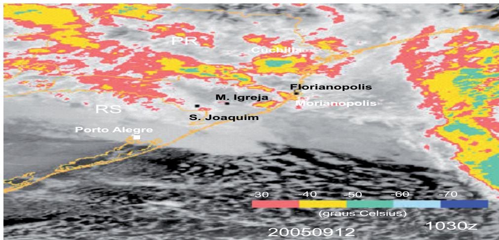
Fig. 6. GOES-12 infrared satellite image of South America from 1030 UTC 12 September 2005. The temperature scale °C is show at bottom right.
