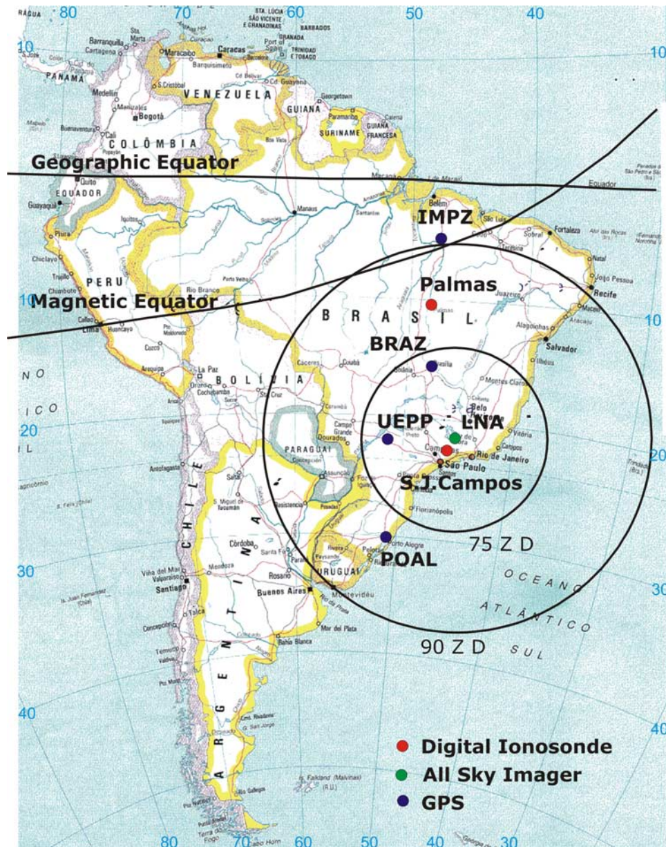
Figure 1. Locations of observatories used to study equatorial plasma depletions. The red points show the two digital ionosonde stations: Palmas (10.2°S, 48.2°) and Sao Jose dos Campos (23.2°S, 45.9°W); the blue points show the four observatories of the Brazilian Network for Continuous Monitoring (“RBMCM”): Imperatriz (IMPZ; 05.29°S, 47.29°W), Brasilia (BRAZ; 15.56°S, 47.52°W), Presidente Prudente (UEPP; 22.07°S, 51.24°W), and Porto Alegre (POAL; 30.04°S, 51.07°W); and the green point shows the all-sky imaging system located at Brazopolis (“LNA”; 22.5°S, 45.6°W). The circles indicate the fields of view at a zenith angle of 75° and 90° projected at a 280-km altitude. Also, the geographic and magnetic equators are shown.
