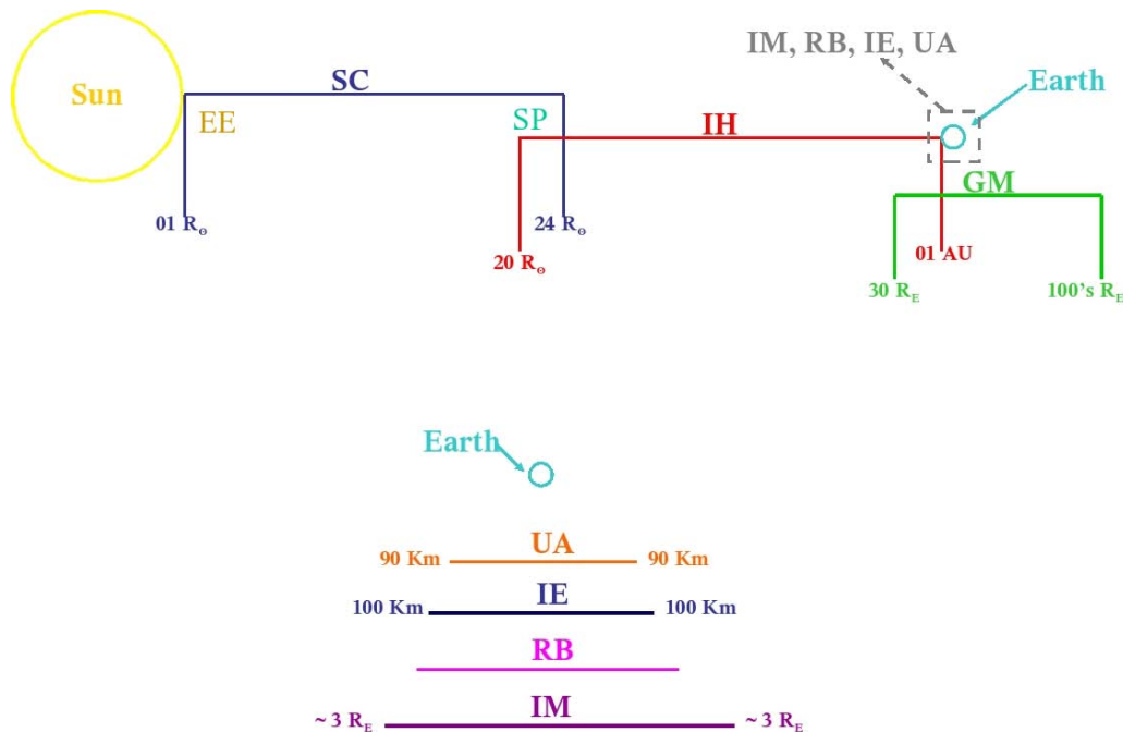
FIGURE 2.2 - Illustration, out of scales, for the domain extension of the SWMF components.
