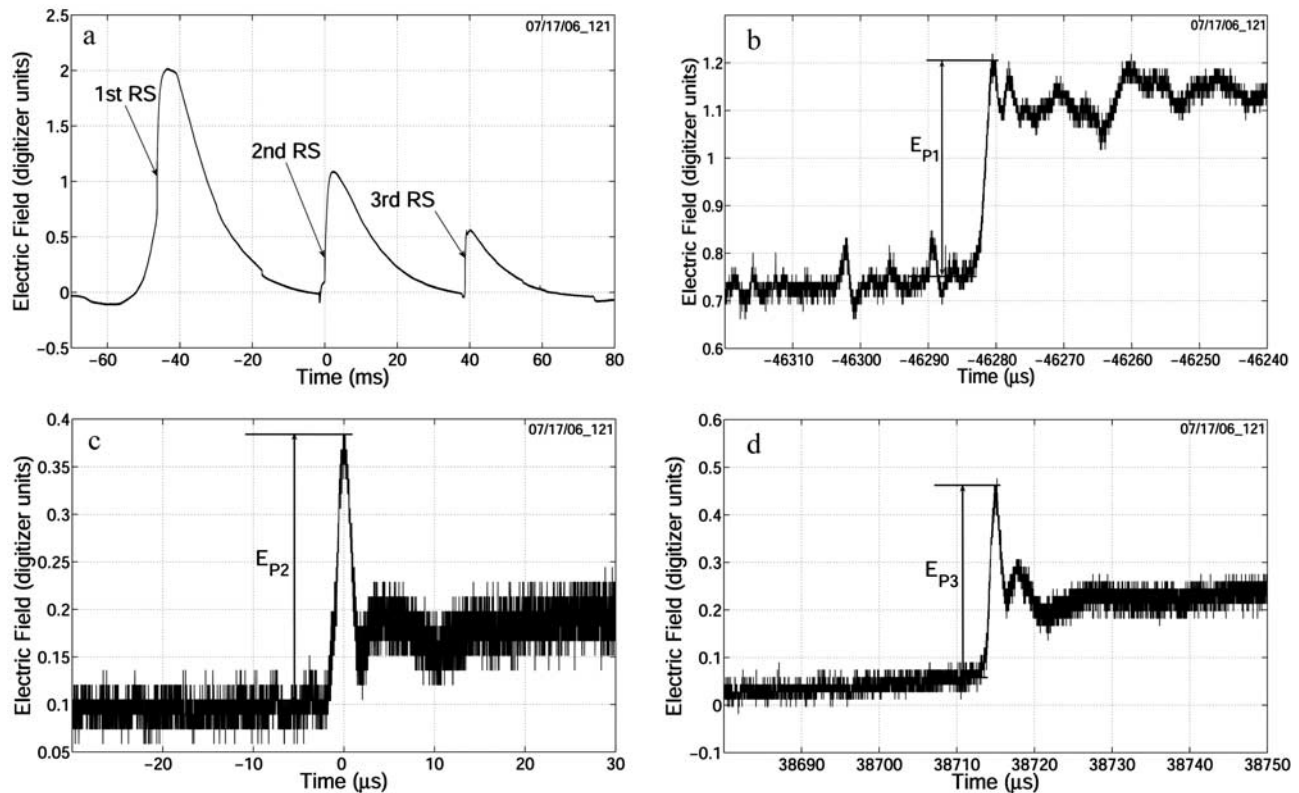
Figure 1. (a). Typical electric field record of a multiple-stroke negative cloud-to-ground flash in Florida with three return strokes (RS) shown on a 150-ms timescale. (b) Electric field of the first return stroke, on an 80- \mu s timescale, of flash shown in Figure 1a. (c) Electric field of the second return stroke, on a 60- \mu s timescale. (d) Electric field of the third return stroke, on a 70- \mu s timescale. Initial (radiation) electric field peaks of return strokes of order 1, 2, and 3 are labeled as E_{P1} , E_{P2} , and E_{P3} , respectively. Note that radiation field peaks seen in Figures 1b–1d are not resolved in Figure 1a.
