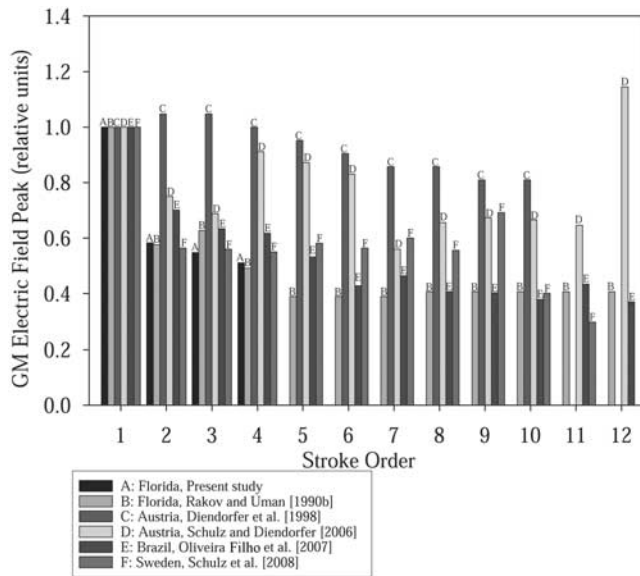
Figure 4. Geometric mean (GM) electric field peaks for strokes of different order estimated from different studies, labeled A, B, C, D, E, and F. For A, field peaks of subsequent strokes of different order are normalized to the electric field peak of the corresponding first return stroke and for B, C, D, E, and F the GM field peaks of subsequent strokes of different order are normalized to the GM field peak for first strokes (including those in single-stroke flashes for B and C). Sample size for strokes of order 12 in study D was as low as three (there were six in study E, and for study B the value is the average for 53 strokes of order 8 through 18).
