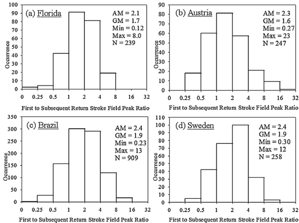
Figure 2. Histogram of the ratio of the first-to-subsequent-return-stroke electric field peak for multiple-stroke negative cloud-to-ground lightning flashes in (a) Florida, (b) Austria, (c) Brazil, and (d) Sweden.
