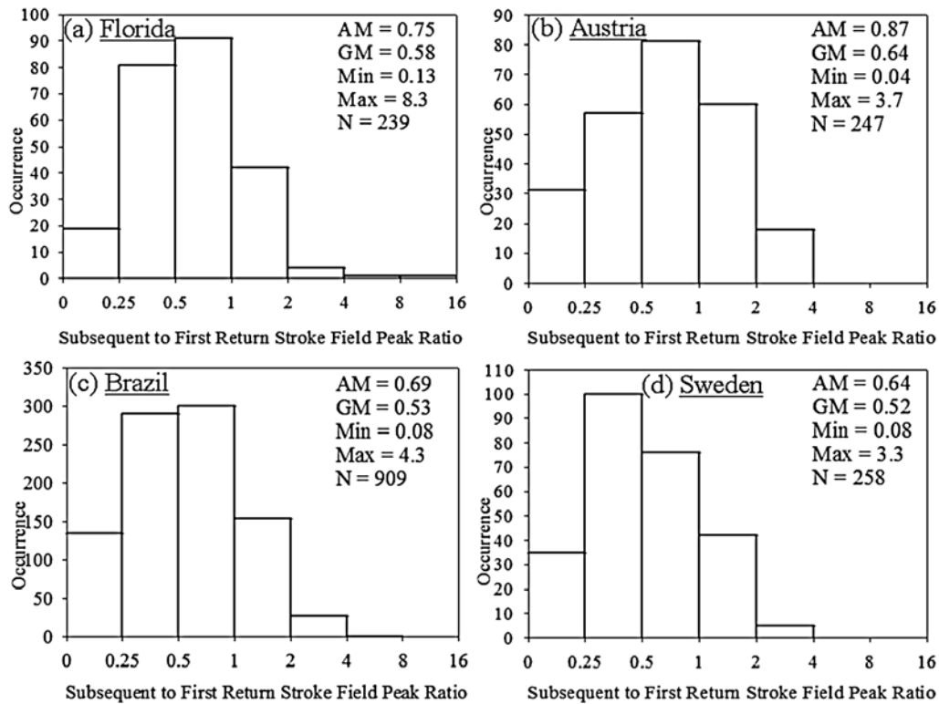
Figure 3. Histogram of the ratio of the subsequent-to-first-return-stroke electric field peak for multiple-stroke negative cloud-to-ground lightning flashes in (a) Florida, (b) Austria, (c) Brazil, and (d) Sweden.
