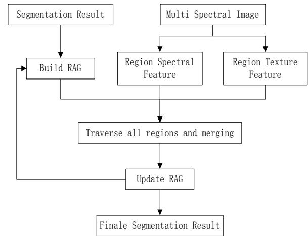
Figure.2 The flow chart of region merging for multi spectral image
