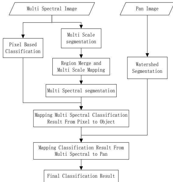
Figure.1 The flow chart of proposed classification method
