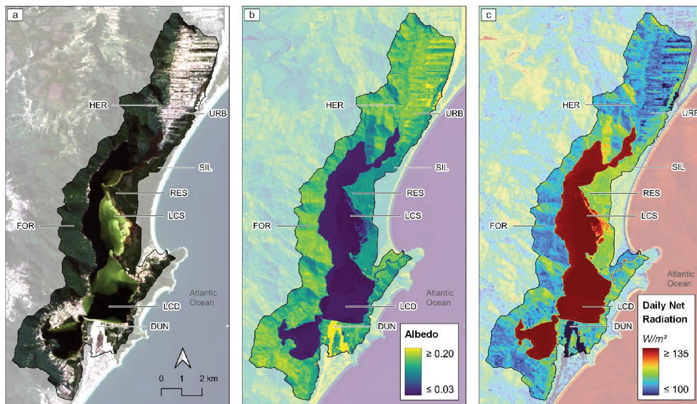
Figure 2. Mean a) true color composite, b) albedo, and c) daily net radiation ( \text{Wm}^{-2} ) over the study area.
