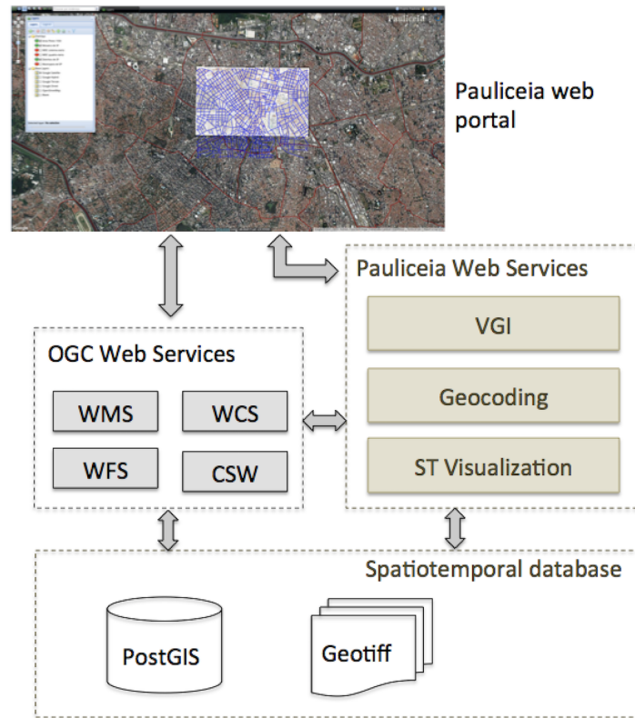
Figure 1. Pauliceia platform architecture
