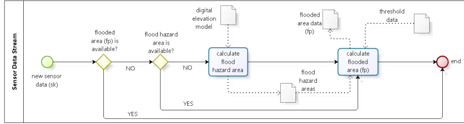
Figure 1. Sensor Data Stream Workflow.
