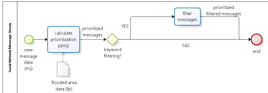
Figure 2. Social Network Message Workflow.
