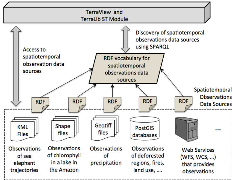
Figure 7. A proposal to access different kinds of spatiotemporal data sources.
