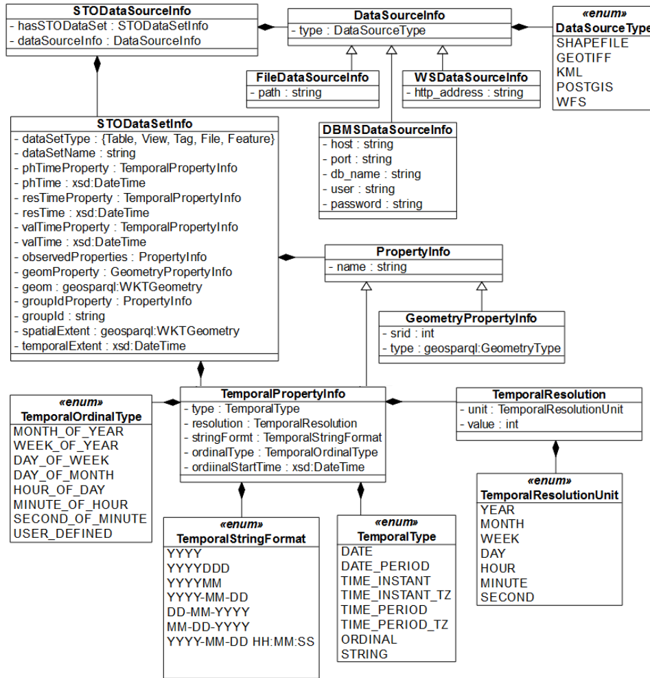
Figure 10. The RDF vocabulary for spatiotemporal observation data sources.
