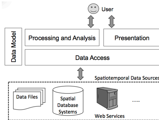
Figure 5. GIS general architecture.
