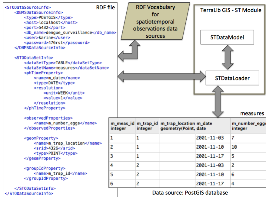
Figure 11. Example of the proposed RDF vocabulary.
