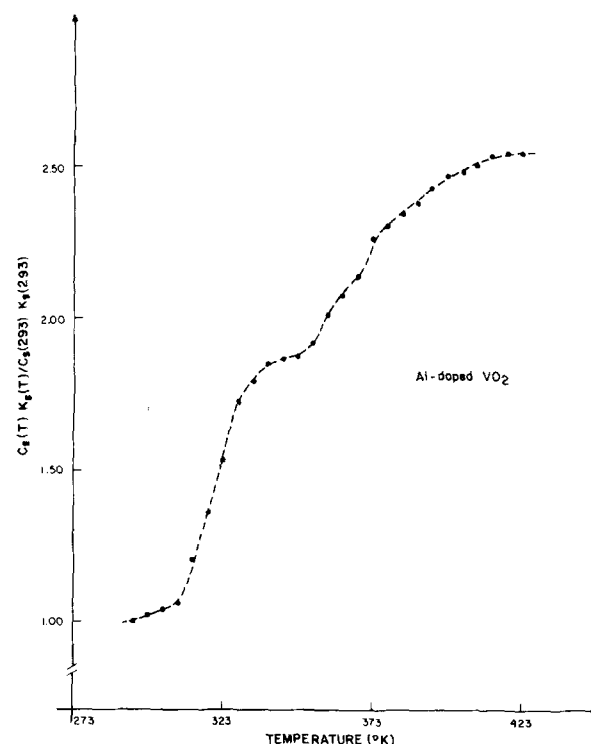
FIG. 6. Temperature variation of C_s(T)K_s(T) of Al-doped \text{VO}_2 , normalized to its value of 293 °K, calculated according to Eq. (3) of the text.
