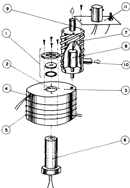
FIG. 4. The PA cell for thermal studies: (1) Window assembly, (2) sample compartment, (3) cell body (anodized aluminium), (4) thermocouple, (5) external heater winding, (6) internal heater winding, (7) cooling assembly, (8) microphone and preamplifier compartment, (9) water inlet, (10) water outlet, and (11) electrical connections.
