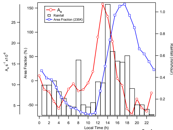
Figure 2: Mean hourly area expansion ( 10^{-6} \text{ s}^{-1} ), rainfall ( \text{mmh}^{-1} ) and 235 K area fraction (%) for the WETAMC/LBA region.
