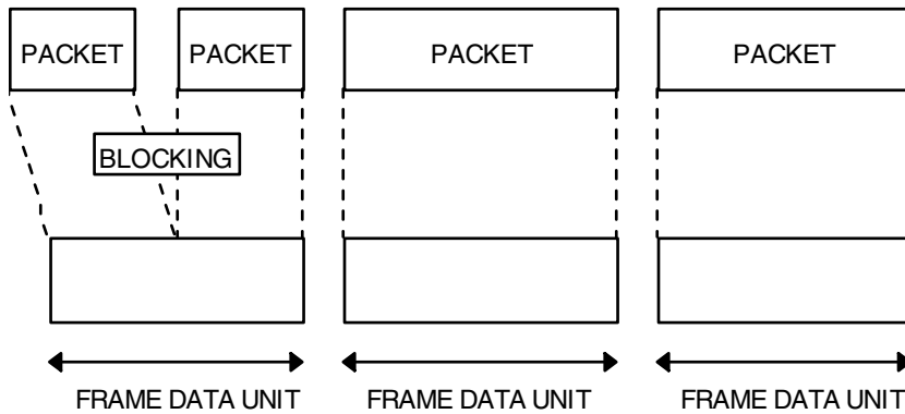
Figure 4-12: Example of VC Packet Processing Procedures
