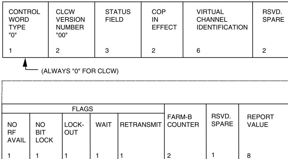
Figure 4-4: Communications Link Control Word
