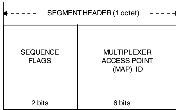
Figure 4-3: Segment Header
