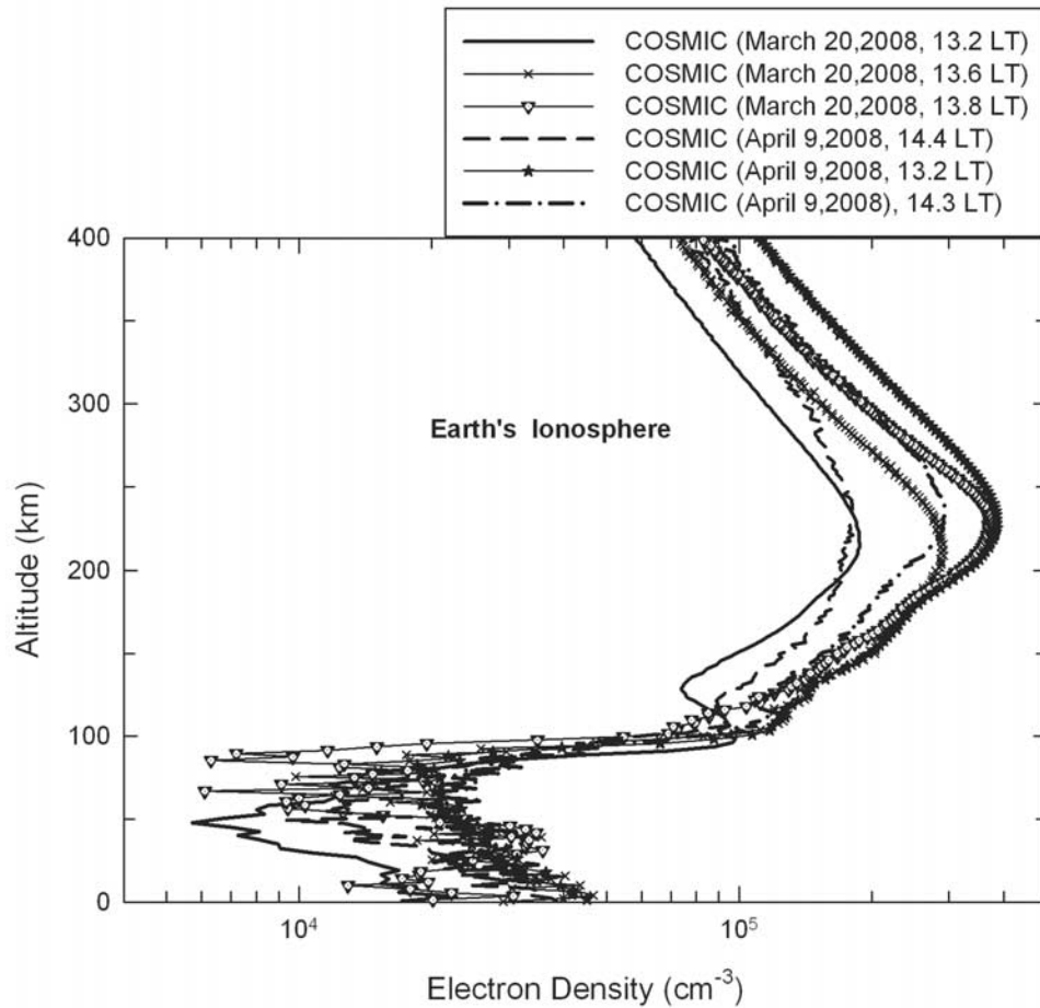
Figure 5. Six sample profiles of electron density representing D , E , and F layers as observed in Earth's ionosphere by radio occultation experiment on board COSMIC satellites at different locations at nearly the same local time in the afternoon.
