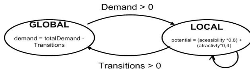
Figure 1. The hybrid Cellular Automata Dynamics
