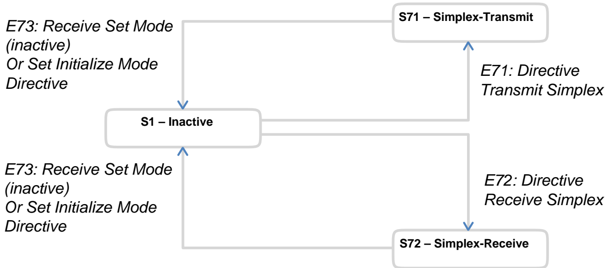
Figure 6-3: Simplex Operations
